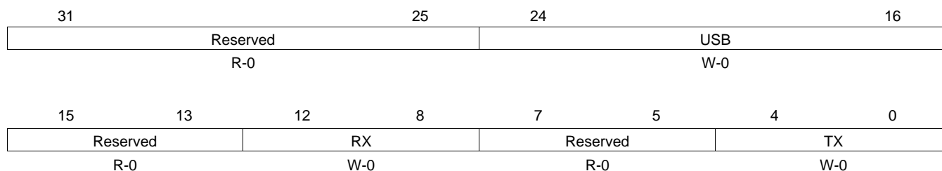
Figure 25. USB Interrupt Mask Clear Register (INTMSKCLRR)
